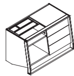
EW25 W1002*D560*H610(mm)
